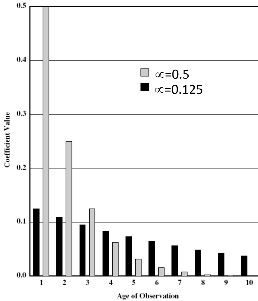
Figure 12.4 Exponential Smoothing Coefficients
